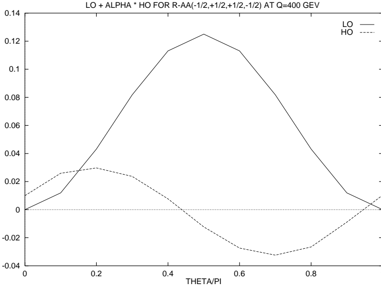
Fig. 8. \theta dependence of LO and HO contribution to R_{AA}(-\frac{1}{2}, +\frac{1}{2}, +\frac{1}{2}, -\frac{1}{2}) for fixed \sqrt{s} = 400\text{GeV} . The HO contribution is given in units of \alpha
