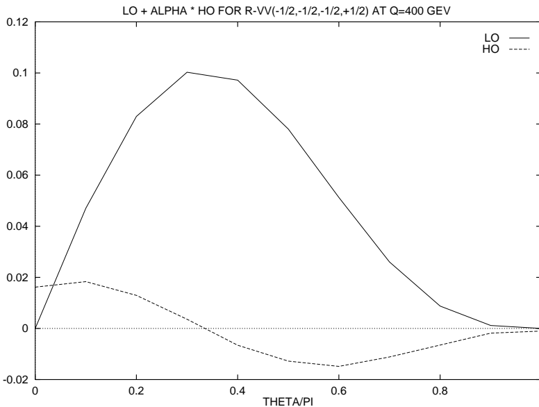
Fig. 7. \theta dependence of LO and HO contribution to R_{VV}(-\frac{1}{2}, -\frac{1}{2}, -\frac{1}{2}, +\frac{1}{2}) for fixed \sqrt{s} = 400\text{GeV} . The HO contribution is given in units of \alpha
