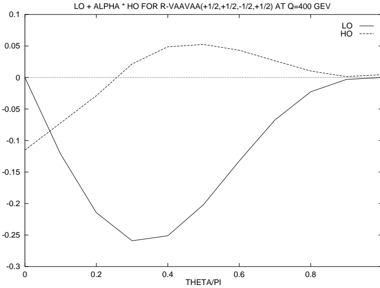
Fig. 9. \theta dependence of LO and HO contribution to R_{VAAVAA}(+\frac{1}{2}, +\frac{1}{2}, -\frac{1}{2}, +\frac{1}{2}) for fixed \sqrt{s} = 400\text{GeV} . The HO contribution is given in units of \alpha
