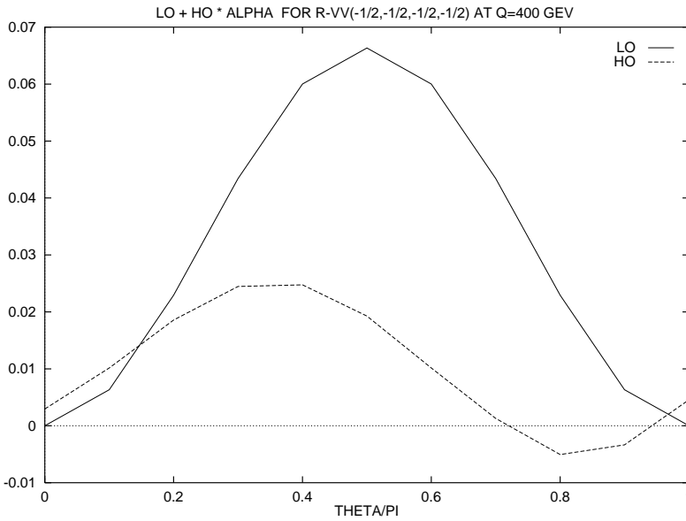
Fig. 6. \theta dependence of LO and HO contribution to R_{VV}(-\frac{1}{2}, -\frac{1}{2}, -\frac{1}{2}, -\frac{1}{2}) for fixed \sqrt{s} = 400\text{GeV} . The HO contribution is given in units of \alpha
