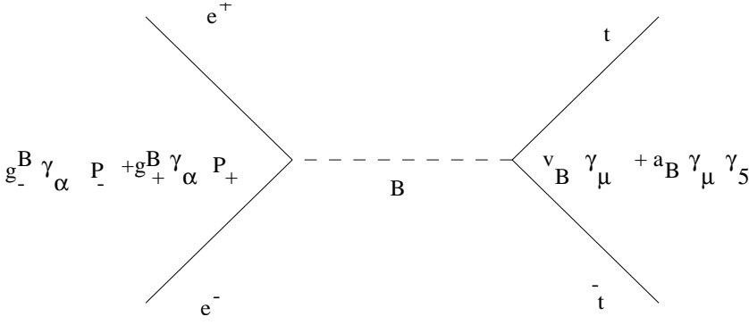
Fig. 1. Definition of the couplings. The symbols P_{\pm} denote the projection operators P_{\pm} = \frac{1}{2}(1 \pm \gamma_5)
