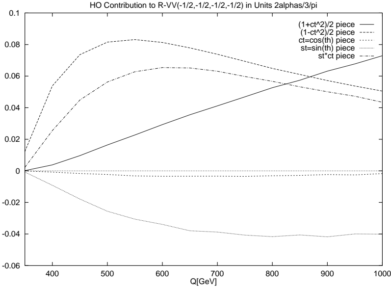
Fig. 2. Energy dependence of the HO contribution to R_{VV}(-\frac{1}{2}, -\frac{1}{2}, -\frac{1}{2}, -\frac{1}{2}) . The HO contribution is decomposed according to (28) and given in units of \alpha . C_1 is denoted by (1+c_t^2)/2 -piece, 2C_2 by (1-c_t^2)/2 -piece, C_3 by c_t -piece, C_4 by s_t -piece and C_5 by s_t c_t -piece
