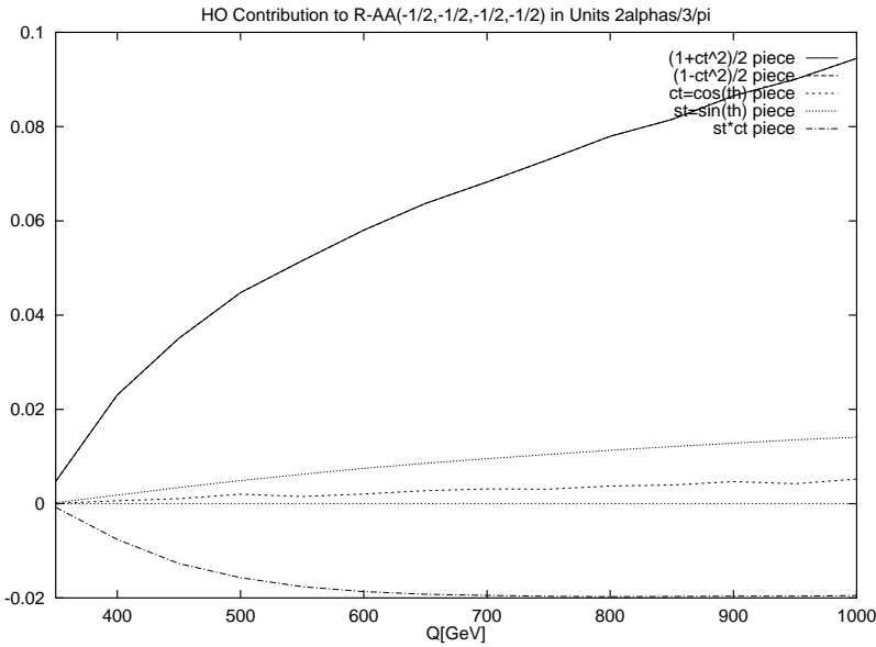
Fig. 3. Energy dependence of the HO contribution to R_{AA}(-\frac{1}{2}, -\frac{1}{2}, -\frac{1}{2}, -\frac{1}{2}) . The HO contribution is decomposed according to (28) and given in units of \alpha . C_1 is denoted by (1+c_t^2)/2 -piece, 2C_2 by (1-c_t^2)/2 -piece, C_3 by c_t -piece, C_4 by s_t -piece and C_5 by s_t c_t -piece
