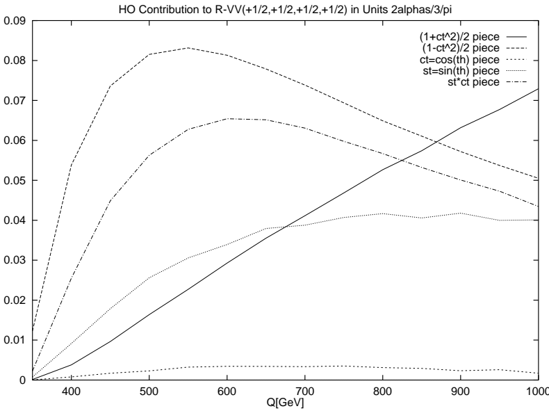
Fig. 5. Energy dependence of the HO contribution to R_{VV}(+\frac{1}{2}, +\frac{1}{2}, +\frac{1}{2}, +\frac{1}{2}) . The HO contribution is decomposed according to (28) and given in units of \alpha . C_1 is denoted by (1 + c_t^2)/2 -piece, 2C_2 by (1 - c_t^2)/2 -piece, C_3 by c_t -piece, C_4 by s_t -piece and C_5 by s_t c_t -piece
